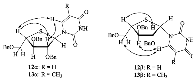
Figure 1. Observed NOE ( \leftrightarrow ) as indicators for the \alpha - and \beta - L -arabino configuration of 12 and 13
